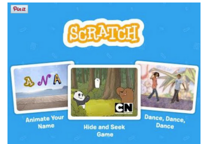
Scratch
